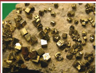
Pyritt
